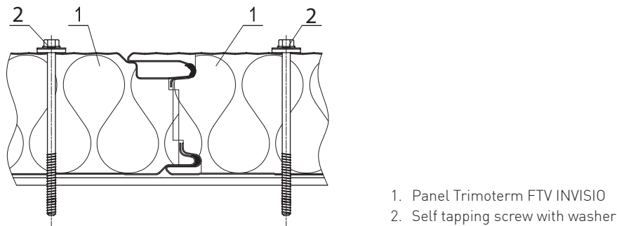
Fig. 14: Edge fixing trough a panel
