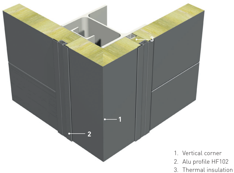
Fig. 39: Detail of a round edge corner.
