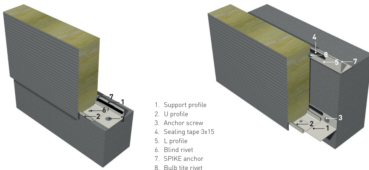
Fig. 30: Detail of attachment to the base beam.
