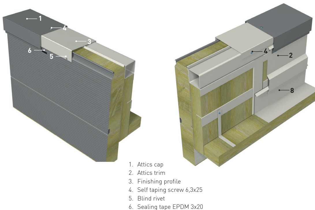
Fig. 36: Detail attics.
