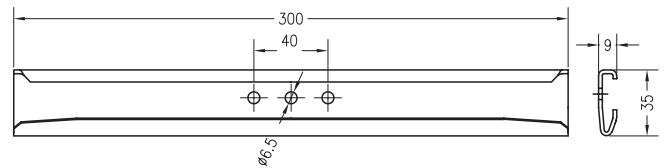
Fig. 11: Spreader bar detail.
