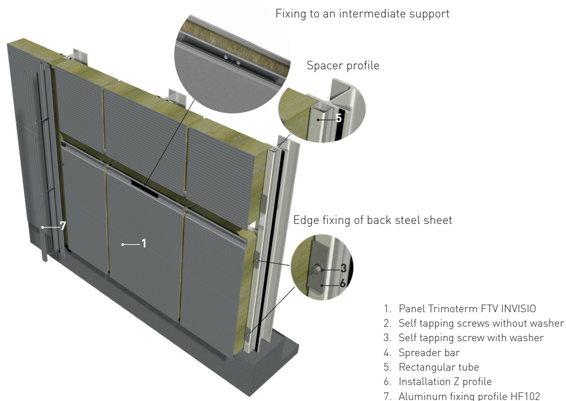
Fig. 9: Horizontal installation with HF102 fixing profile.
