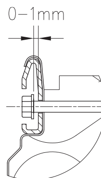
Figure 47: Recommended fixing of intermediate support.
