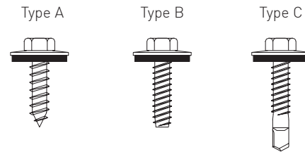
Fig. 19: Fixing screw types.
